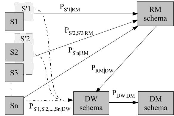
Fig. 2. Proposed architecture.
