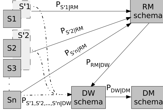
Fig. 3. Proposed architecture.
